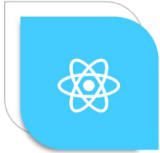
React Native
