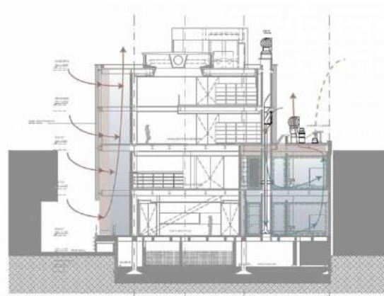
Natural air extraction
