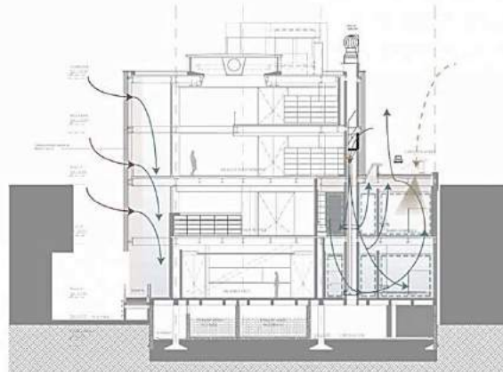
Natural air ventilation
