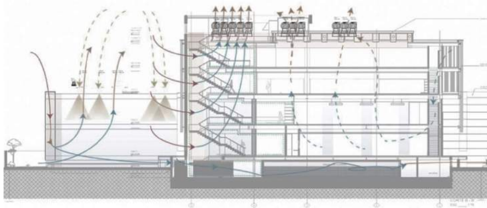
Natural air extraction
