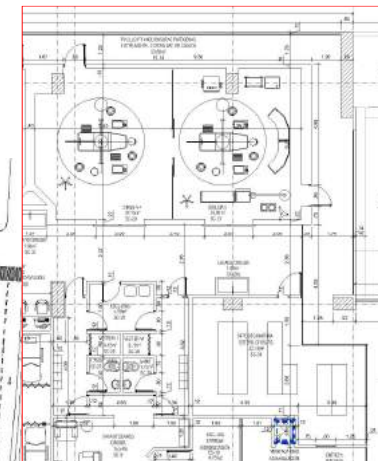
Det: Surgery- Sterilization Cleaing hall
