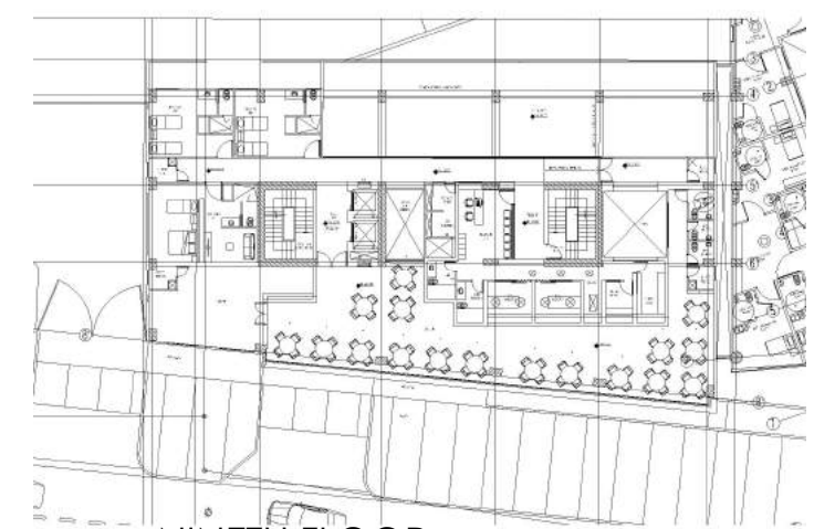
NINETH FLOOR SPA-RESTAURANT-ROOMS
