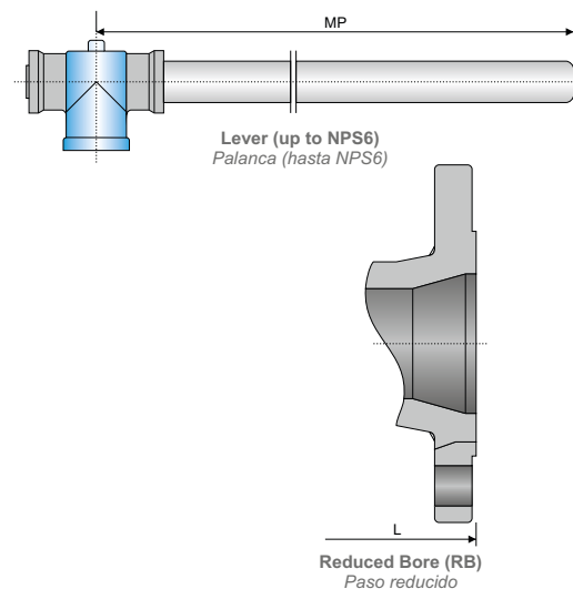
Butt Weld (BW) Soldadura a tope
