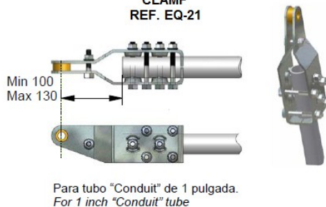
BRIDA/ CLAMP REF. EQ-21
