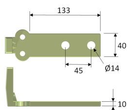
TERMINALES CON NEMA 2/ TWO-HOLE NEMA TERMINALS
