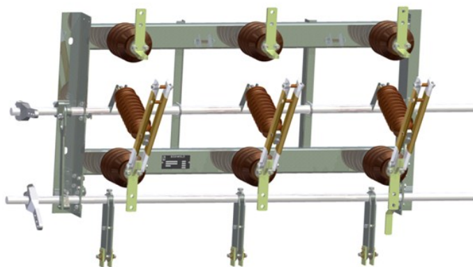
SECCIONADOR TRIPOLAR CON PORTAFUSIBLES/ THREE-POLE DISCONNECT SWITCH WITH FUSE BASES REFERENCIA/ REFERENCE: PF
