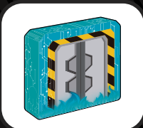
Firewall
