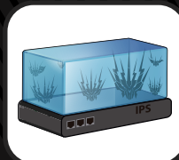
IPS
